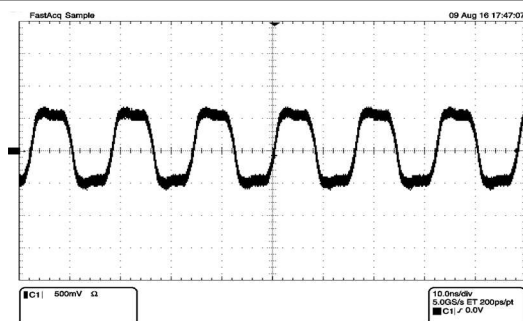
图 7-18. 100BASE-TX PMD Eye Waveform
