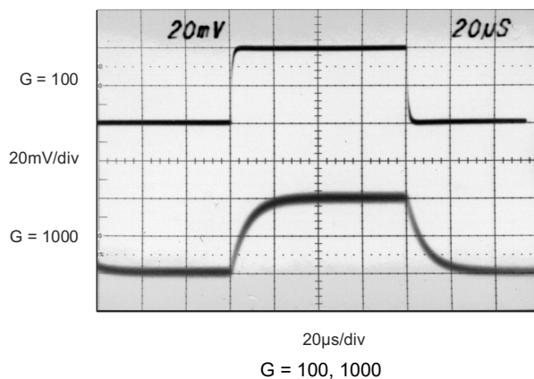
图 7-20. Small Signal
