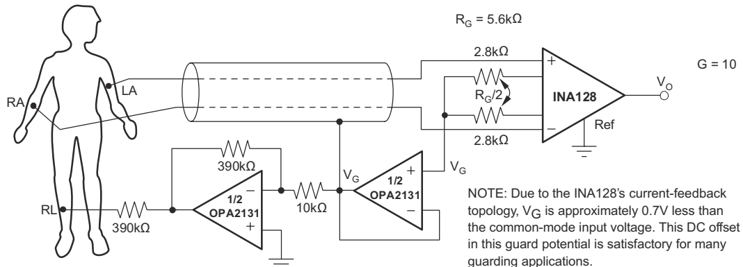
图 9-12. ECG Amplifier With Right-Leg Drive
