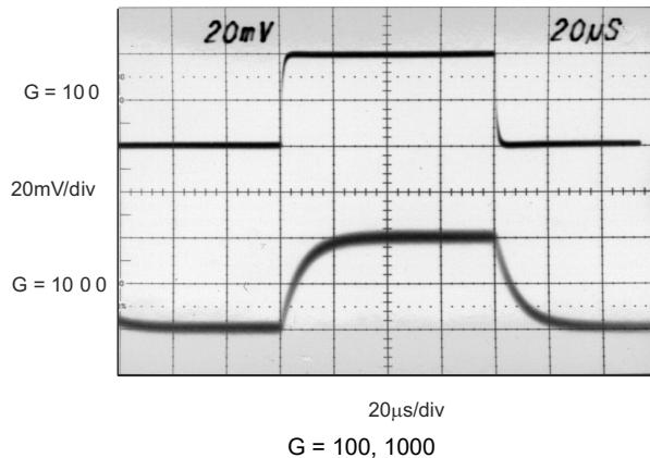
图 9-5. Small Signal
