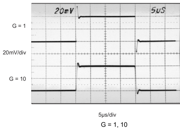
图 7-19. Small Signal
