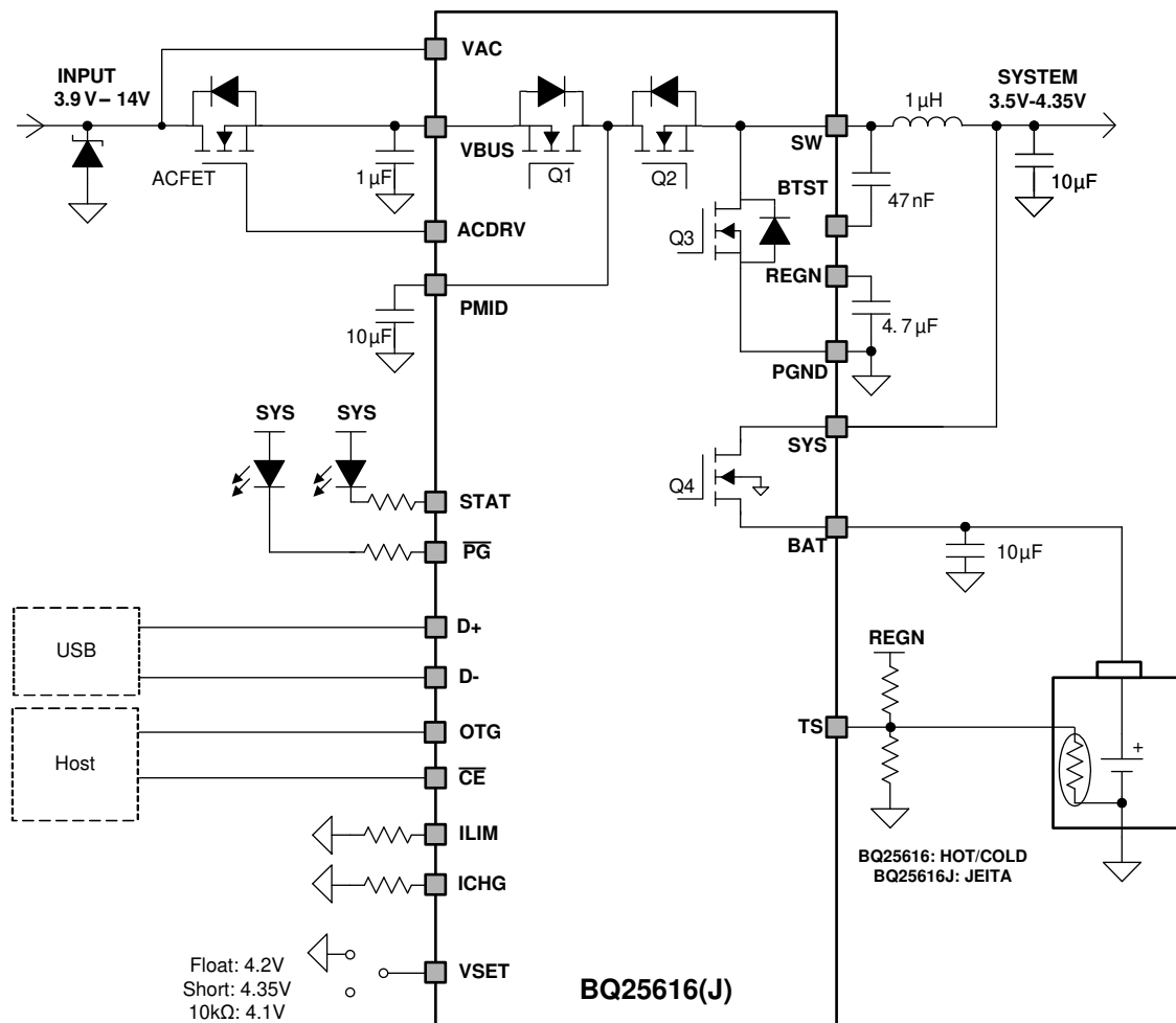
图 10-22. BQ25616/616J Application Diagram with External OVP
