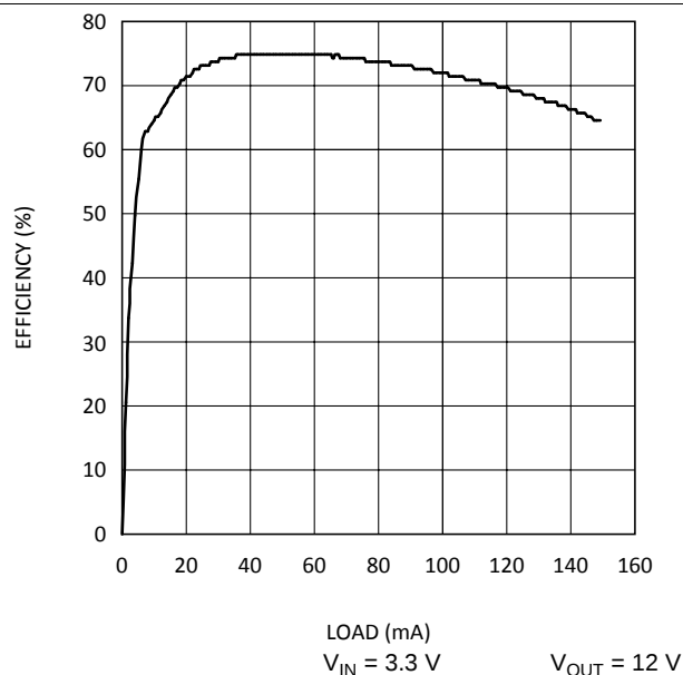
Figure 33. Efficiency vs Load Current - X Option
