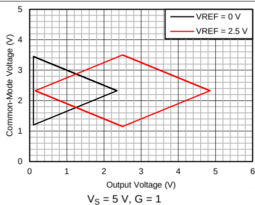
图 55. Input Common-Mode Voltage vs Output Voltage
