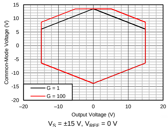
图 58. Input Common-Mode Voltage vs Output Voltage
