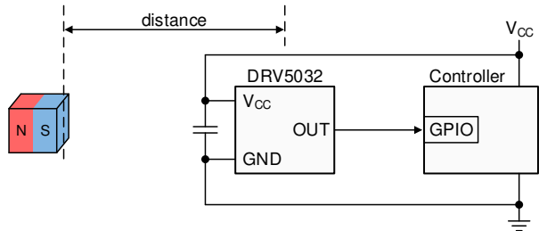
Copyright © 2017, Texas Instruments Incorporated 典型电路原理图
