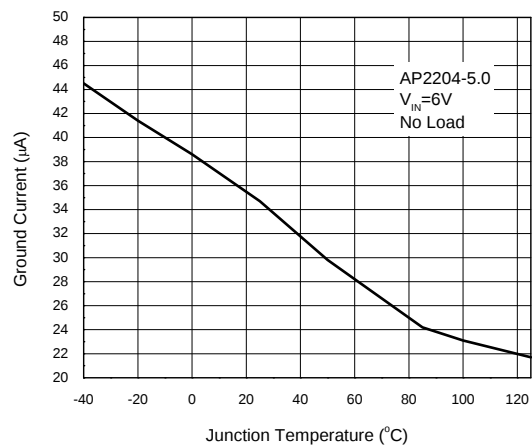
Ground Current vs. Junction Temperature
