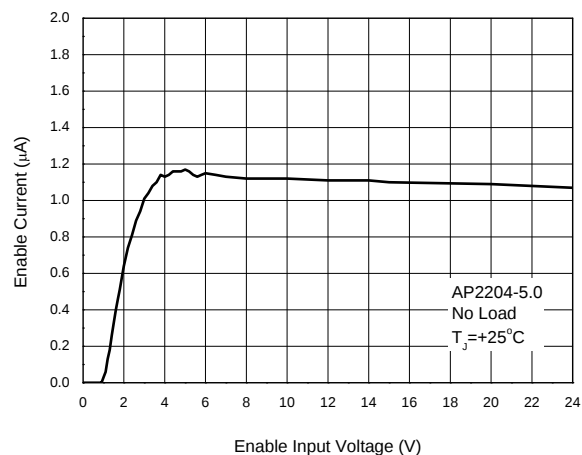
Enable Current vs. Enable Input Voltage
