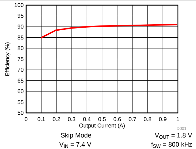
图 14. Efficiency vs Output Current, SKIP Mode
