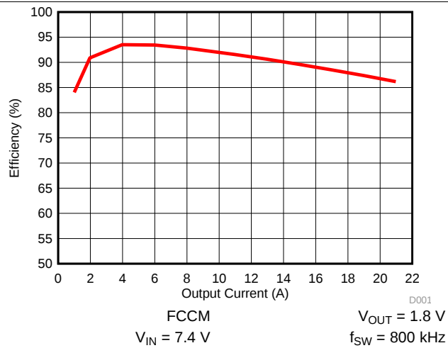
图 13. Efficiency vs Output Current, FCCM
