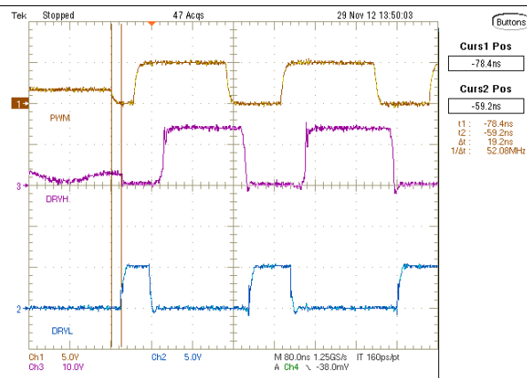
图 4. DRVH Low to DRVH High
