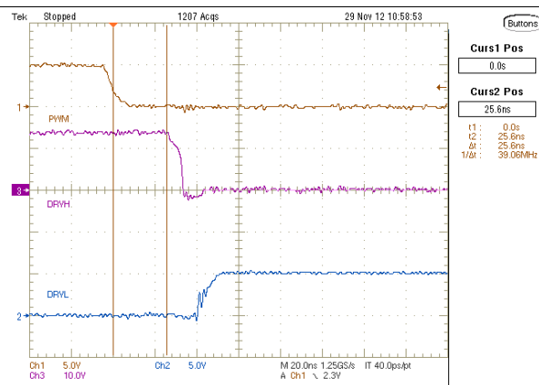
图 2. PWM Low to DRVH Low
