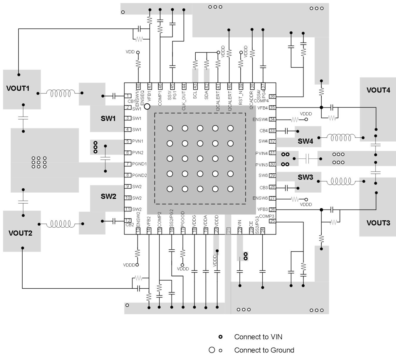
Figure 46. Layout Schematic
