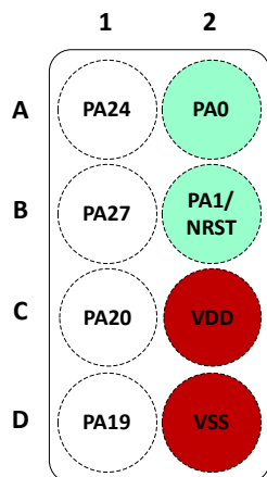
图 6-8. 8-Pin YCJ (DSBGA) (Bumps Down View)
