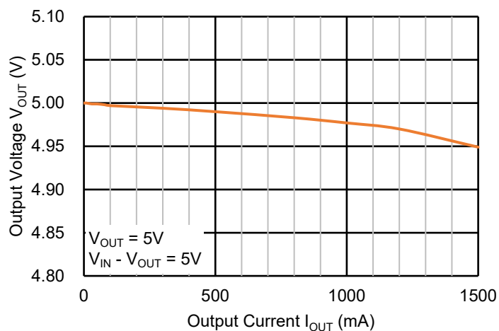
5V Output Load Regulation
