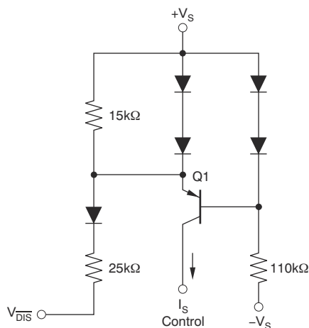
图 7-4. Simplified Disable Control Circuit
