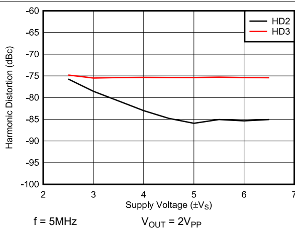
图 6-8. Harmonic Distortion vs Supply Voltage
