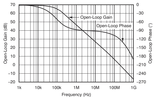
图 6-60. Open-Loop Gain and Phase
