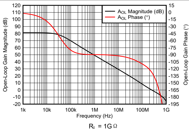
图 6-21. Open-Loop Gain Magnitude and Phase vs Frequency
