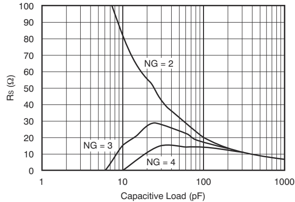
图 8-3. Required R_S vs Noise Gain
