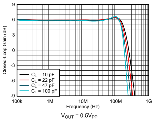
图 6-36. Frequency Response vs Capacitive Load
