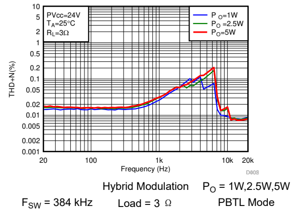
图 7-28. THD+N vs Frequency-PBTL
