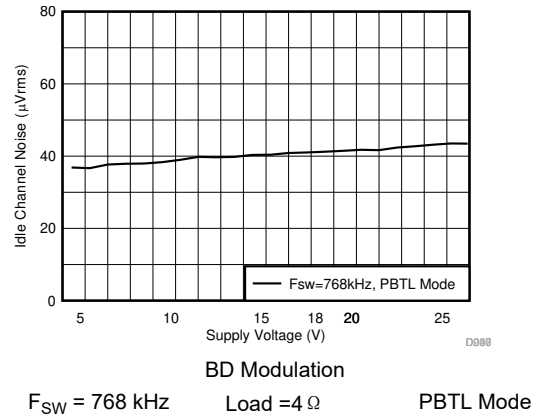
图 7-77. Idle Channel Noise vs Supply Voltage
