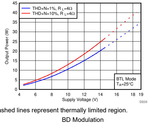
图 7-55. Output Power vs Supply Voltage
