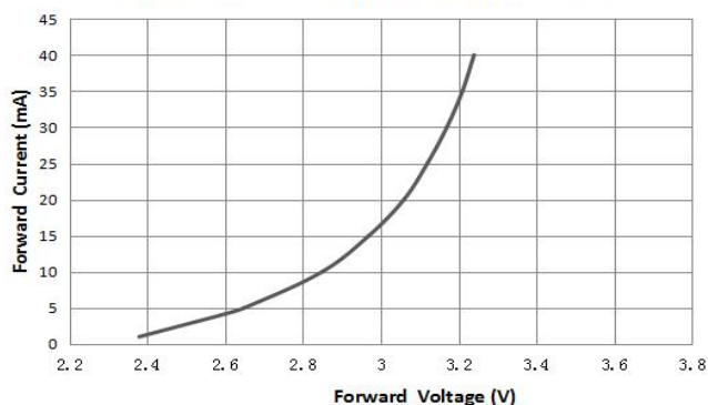
伏安特性曲线 Forward Current VS. Forward Voltage ( T_a=25^\circ\text{C} )
