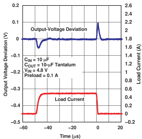
图 6-7. TLV1117-33 Load Transient Response
