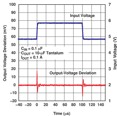
图 6-8. TLV1117-33 Line Transient Response
