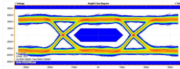
图 7-2. 3.4 Gbps HDMI 1.4 Eye Diagram in DCK Package
