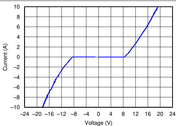
图 5-3. TLP Plot IO to GND
