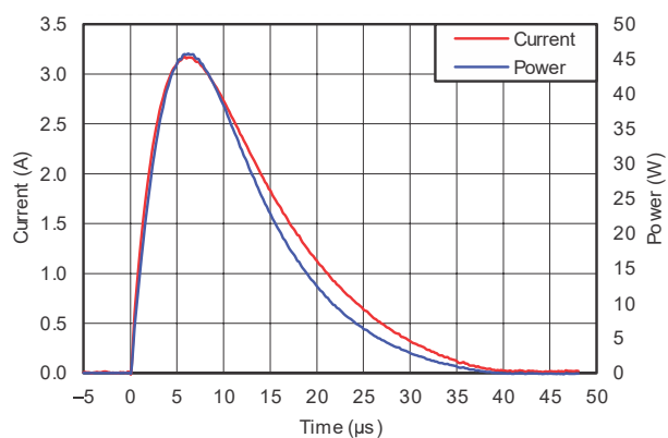
图 5-2. Surge Curve ( t_p = 8/20 \mu s , Pin IO to GND)
