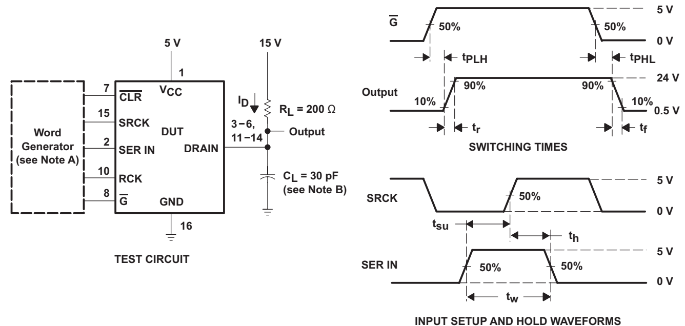
Figure 8. Resistive-Load Test Circuit and Voltage Waveforms
