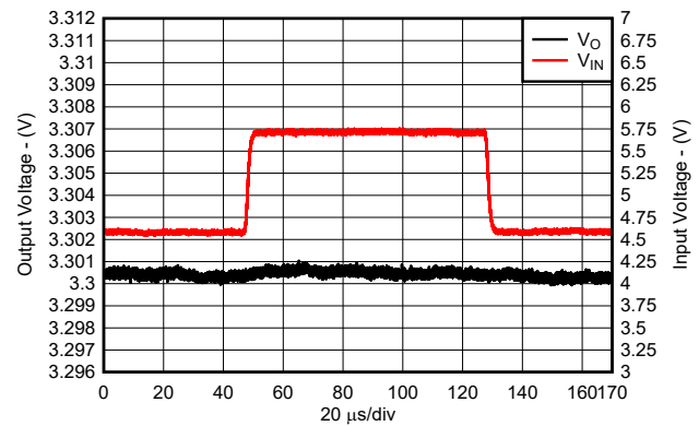
图 7-17. Line Transient Response (New Chip)
