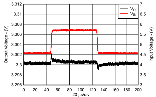
图 7-19. Line Transient Response (New Chip)
