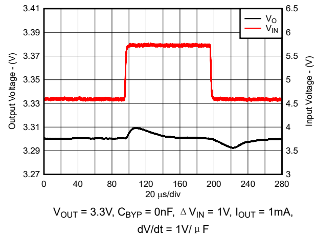
图 7-15. Line Transient Response (New Chip)
