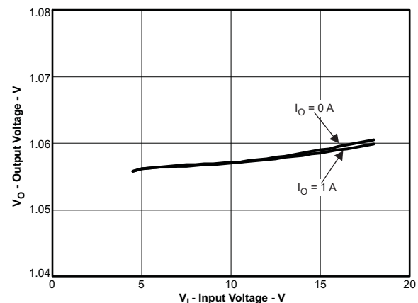
Figure 9. 1.05-V Output Voltage vs Input Voltage
