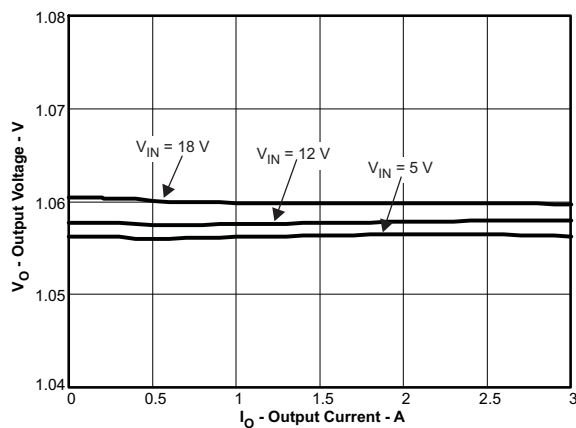
Figure 8. 1.05-V Output Voltage vs Output Current
