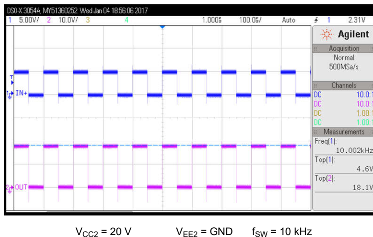
图 9-6. PWM Input and Gate Voltage Waveform
