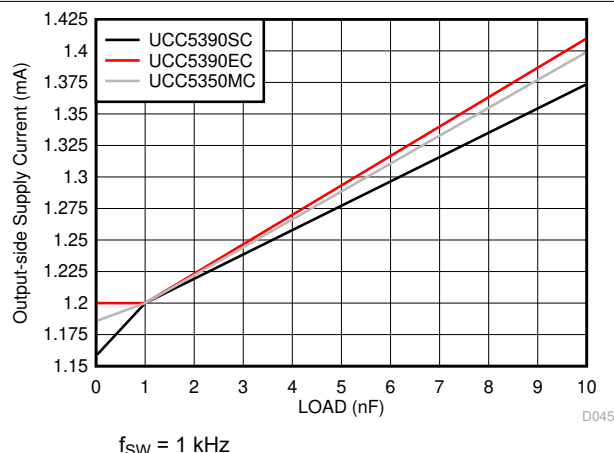
图 6-23. I_{CC2} Supply Current vs Load Capacitance
