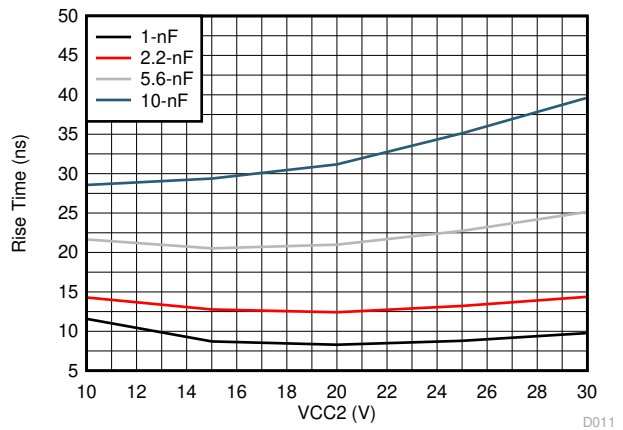
图 6-38. UCC5350SBD Rise Time vs C_L and V_{CC2}
