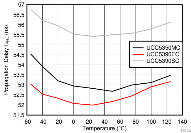
图 6-35. Propagation Delay t_{PHL} vs Temperature
