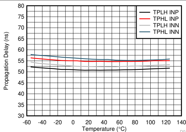
图 6-33. UCC5350SBD Propagation Delay vs Temperature
