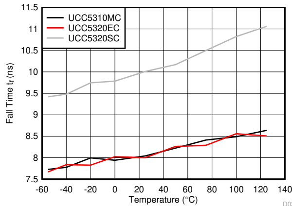
图 6-29. Fall Time Vs Temperature
