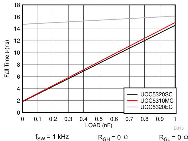
图 6-39. Fall Time vs Load Capacitance
