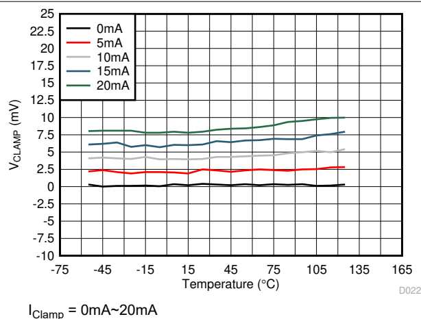
图 6-25. UCC5350M V_{Clamp} vs Temperature
