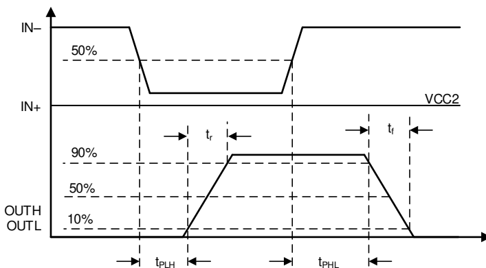
图 7-2. t_{OUTH} and t_{OUTL} Propagation Delay, Inverting Configuration
