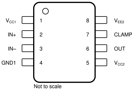
图 5-2. UCC5310M and UCC5350M 8-Pin SOIC Top View
