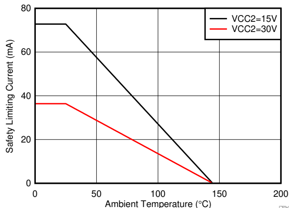
图 6-1. Thermal Derating Curve for Limiting Current per VDE for D Package
