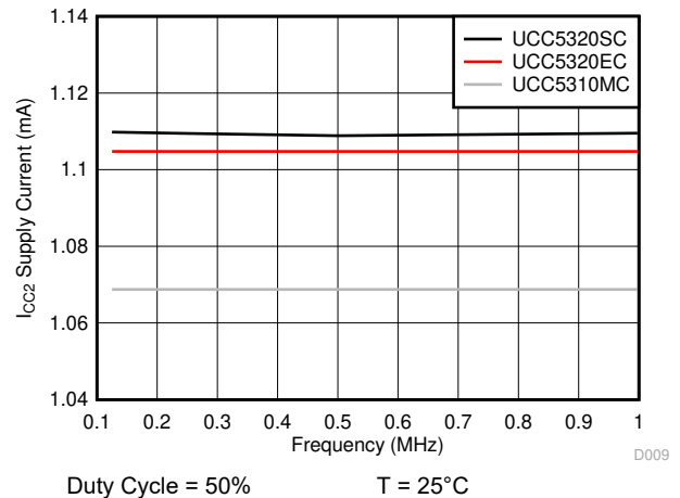
图 6-20. I_{CC2} Supply Current vs Input Frequency
