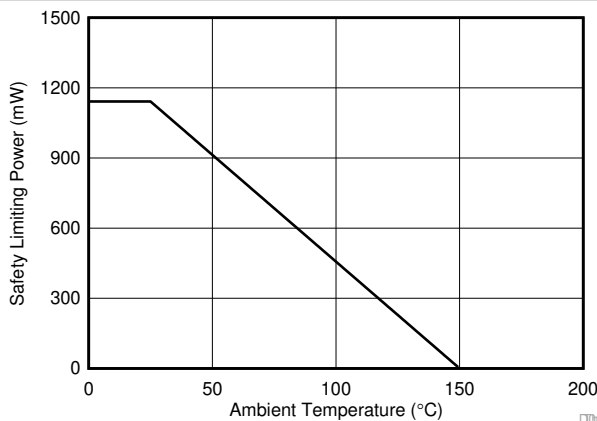
图 6-3. Thermal Derating Curve for Limiting Power per VDE for D Package
