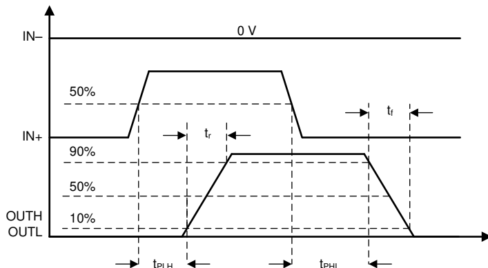
图 7-1. t_{OUTH} and t_{OUTL} Propagation Delay, Noninverting Configuration
