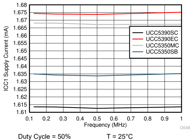
图 6-15. I_{CC1} Supply Current vs Input Frequency
