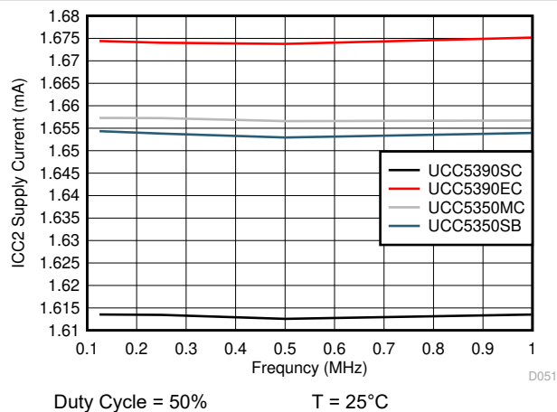
图 6-21. I_{CC2} Supply Current vs Input Frequency
