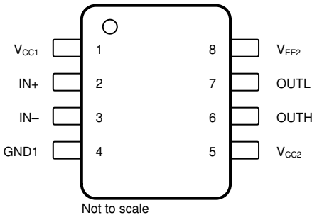
图 5-1. UCC5320S, UCC5350SB, and UCC5390S 8-Pin SOIC Top View
