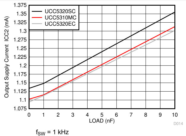
图 6-22. I_{CC2} Supply Current vs Load Capacitance
