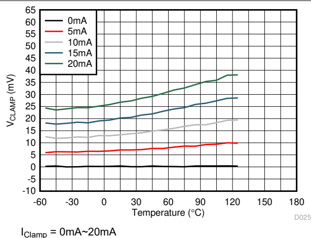
图 6-24. UCC5310M V_{Clamp} vs Temperature
