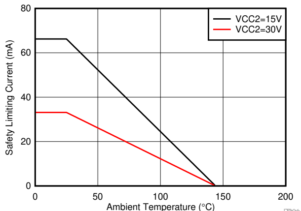
图 6-2. Thermal Derating Curve for Limiting Current per VDE for DWV Package
