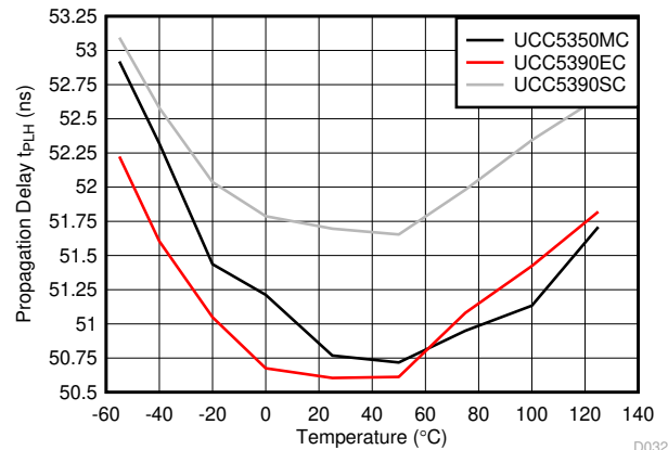
图 6-32. Propagation Delay t_{PLH} vs Temperature
