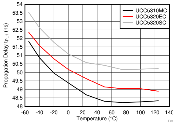
图 6-31. Propagation Delay t_{PLH} vs Temperature
