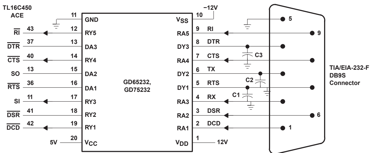
图 7-2. Typical Connection
