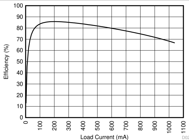
图 6-24. Efficiency vs Load Current
