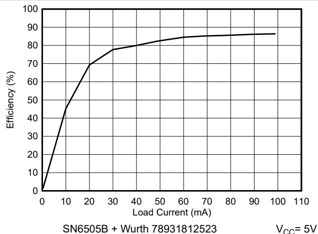
图 6-40. Efficiency vs Load Current
