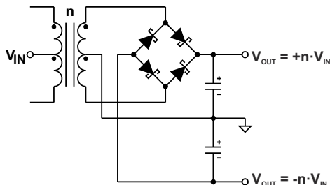
图 9-9. Bridge Rectifier With Center-Tapped Secondary Enables Bipolar Outputs
