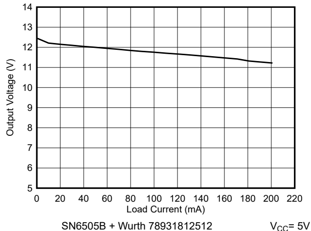
图 6-41. Output Voltage vs Load Current
