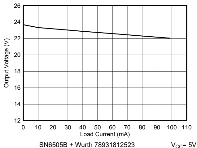
图 6-39. Output Voltage vs Load Current
