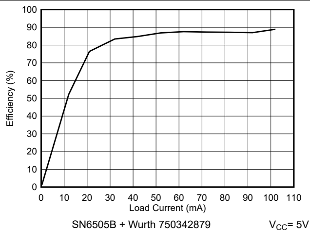
图 6-32. Efficiency vs Load Current
