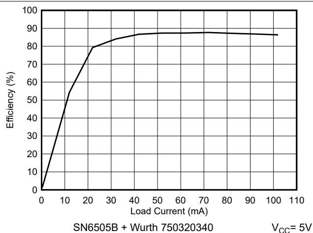
图 6-34. Efficiency vs Load Current
