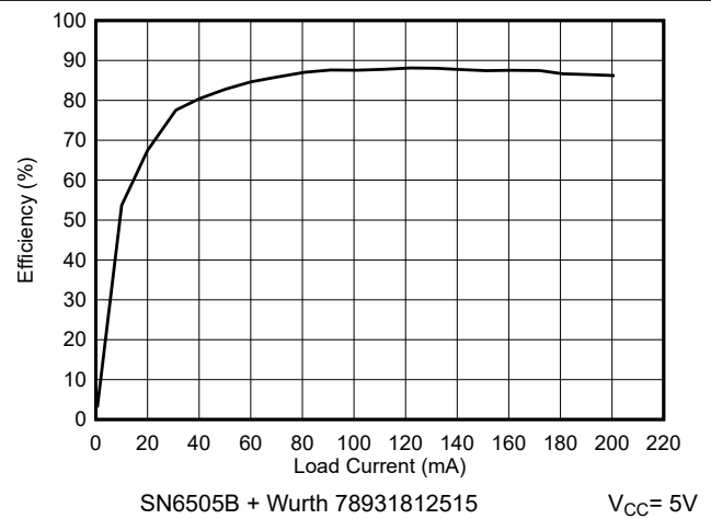
图 6-44. Efficiency vs Load Current
