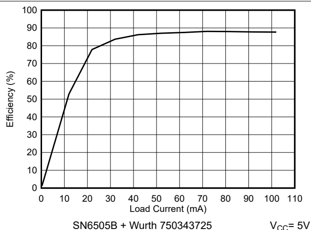
图 6-38. Efficiency vs Load Current
