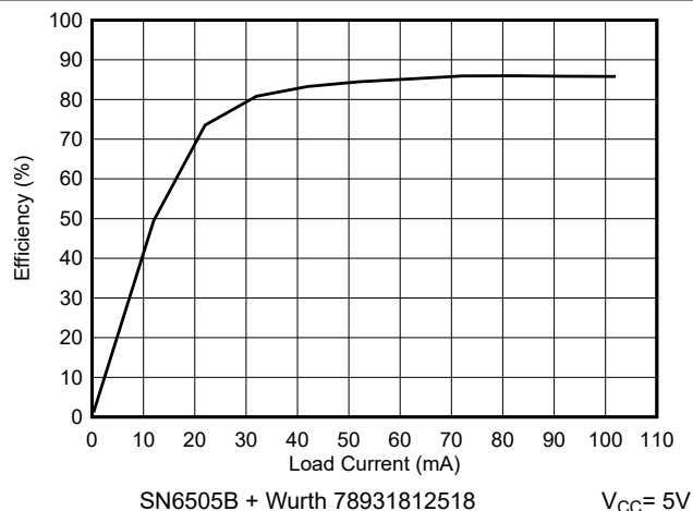
图 6-36. Efficiency vs Load Current
