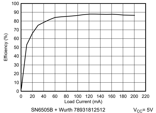
图 6-42. Efficiency vs Load Current
