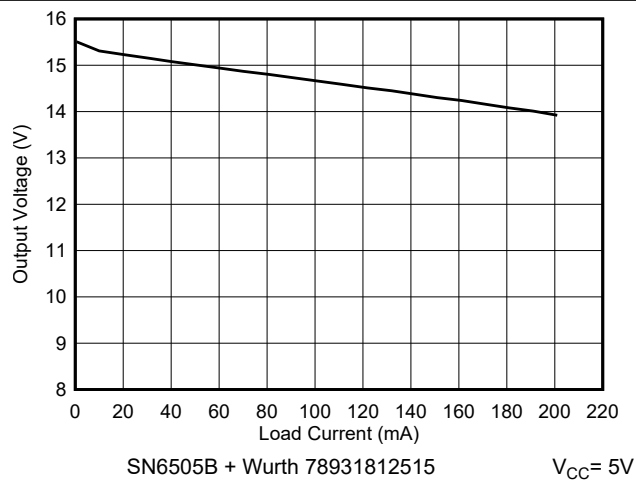
图 6-43. Output Voltage vs Load Current
