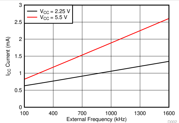
图 6-46. Current vs External Frequency
