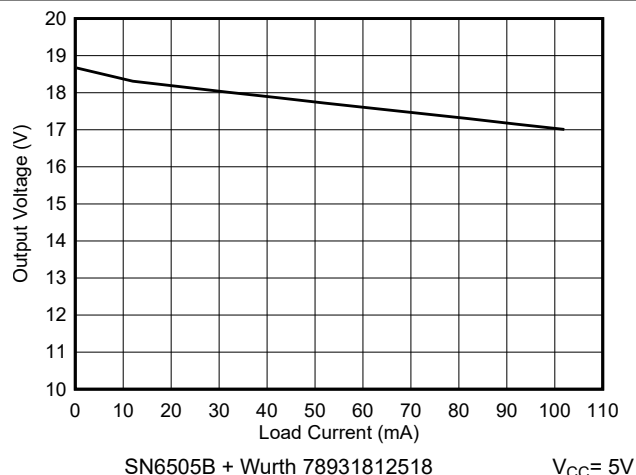
图 6-35. Output Voltage vs Load Current
