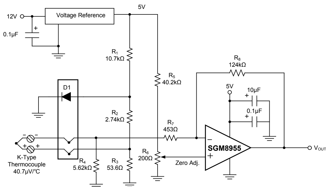
Figure 3. Temperature Measurement
