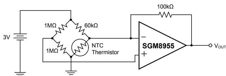
Figure 7. Thermistor Measurement
