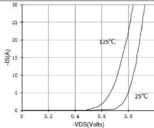
Figure 6. Body-Diode Characteristics
