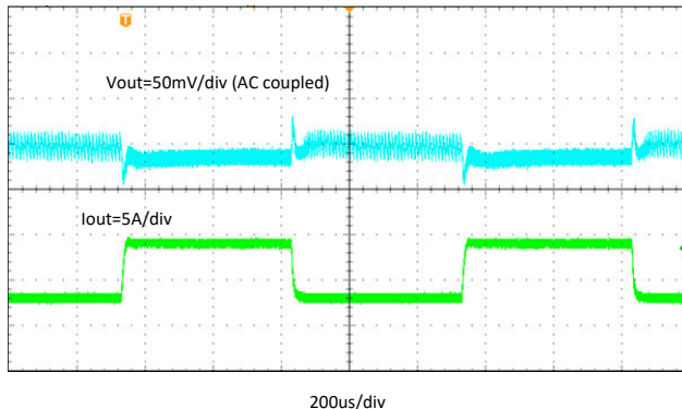
图 7-20. TPS566231 Transient Response
