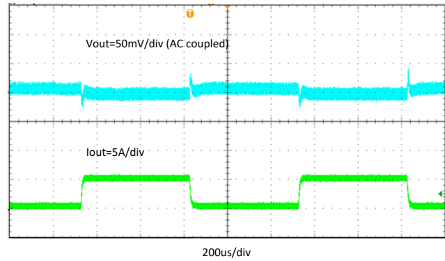
图 7-21. TPS566238 Transient Response
