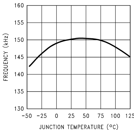
Figure 7-12. Switching Frequency
