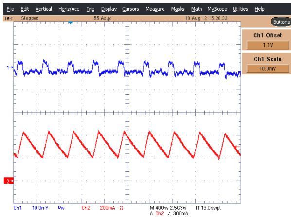
图 65. DCDCx Voltage Ripple and Inductor Current at 300 mA Load, 1.1-V V_{OUT}
