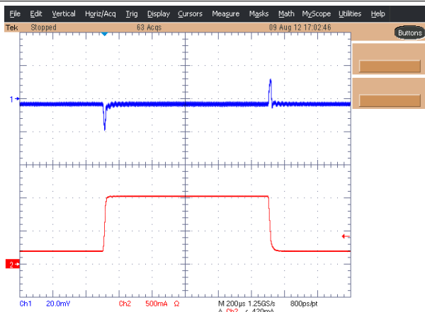
图 75. DCDCx Load Transient Response, 1.5 V OUT , 200-1000-200 mA Load
