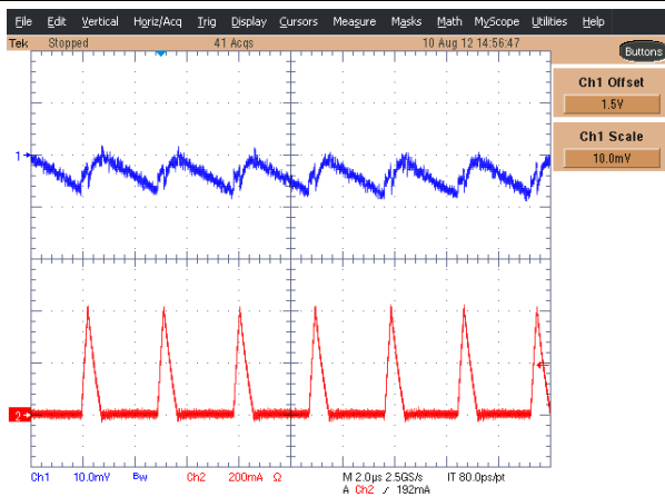
图 67. DCDCx Voltage Ripple and Inductor Current at 50 mA Load, 1.5-V V_{OUT}
