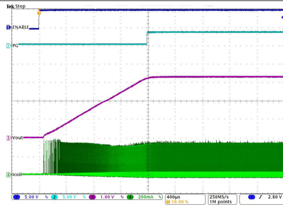
Figure 32. Startup into 100 mA
