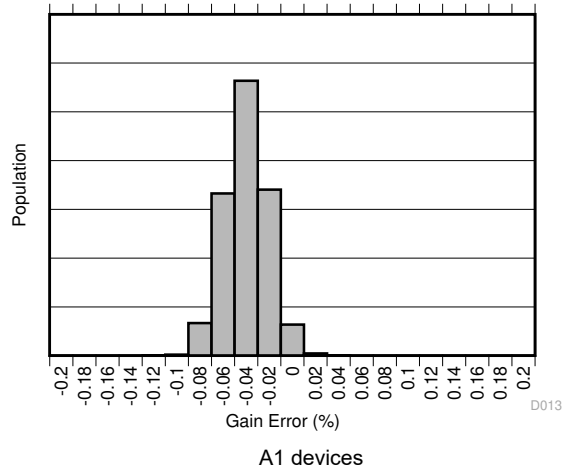
图 6-5. Gain Error Production Distribution
