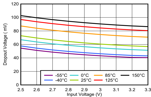
V_{OUT} = 3.3\text{ V} , I_{OUT} = 10\text{ mA} Figure 5-5. V_{DO} vs V_{IN}
