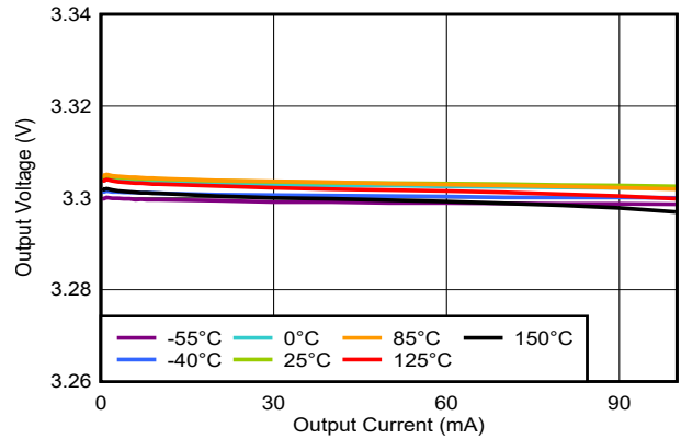
V_{IN} = 4.3\text{ V} , V_{OUT} = 3.3\text{ V} , 0\text{ mA} \leq I_{OUT} \leq 100\text{ mA} Figure 5-2. Load Regulation
