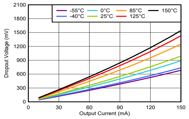
V_{OUT} = 3.3\text{ V} Figure 5-6. V_{DO} vs I_{OUT}
