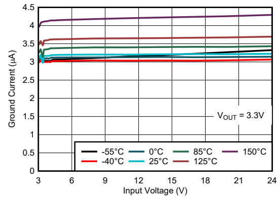
Figure 5-8. Ground Current vs V_{IN}
