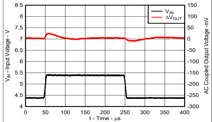
Figure 5-14. V_{IN} Line Transient Response (4.3 V to 5.3 V)
