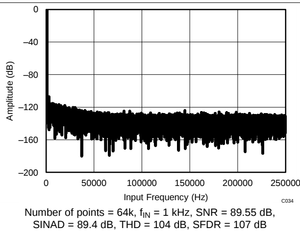
Figure 34. Typical FFT Plot ( 1.25 \times V_{REF} )
