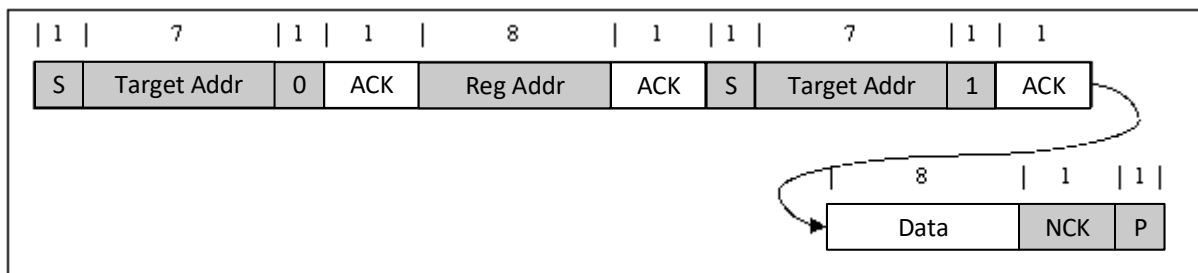
图 9-16. Single Read
