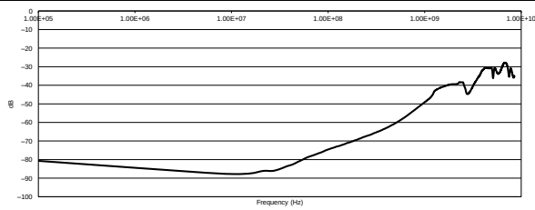
Figure 1. Differential S21 vs Frequency for Port A
