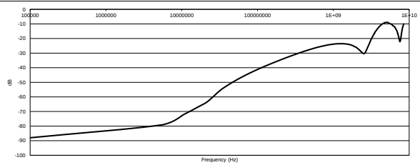
Figure 3. XTALK Port A
