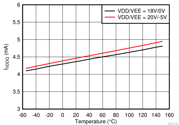
图 6-9. I_{VDDQ} Supply Current vs Temperature
