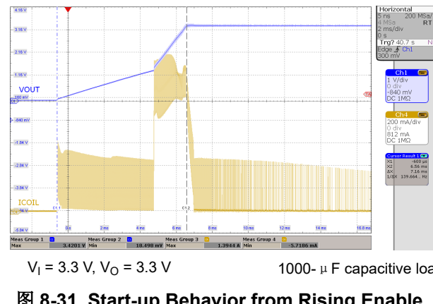
图 8-31. Start-up Behavior from Rising Enable
