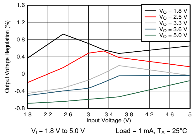
图 8-19. Line Regulation
