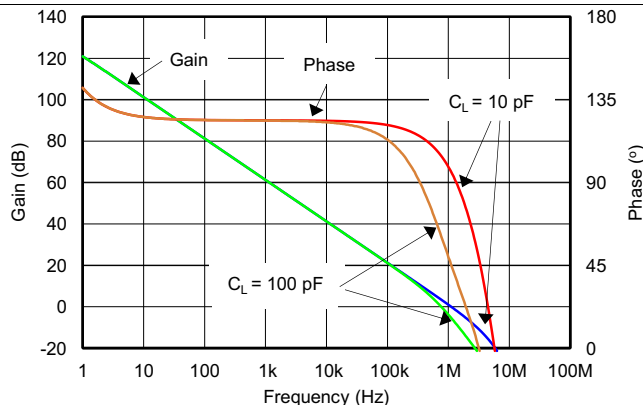
图 1. Open-Loop Gain and Phase vs Frequency
