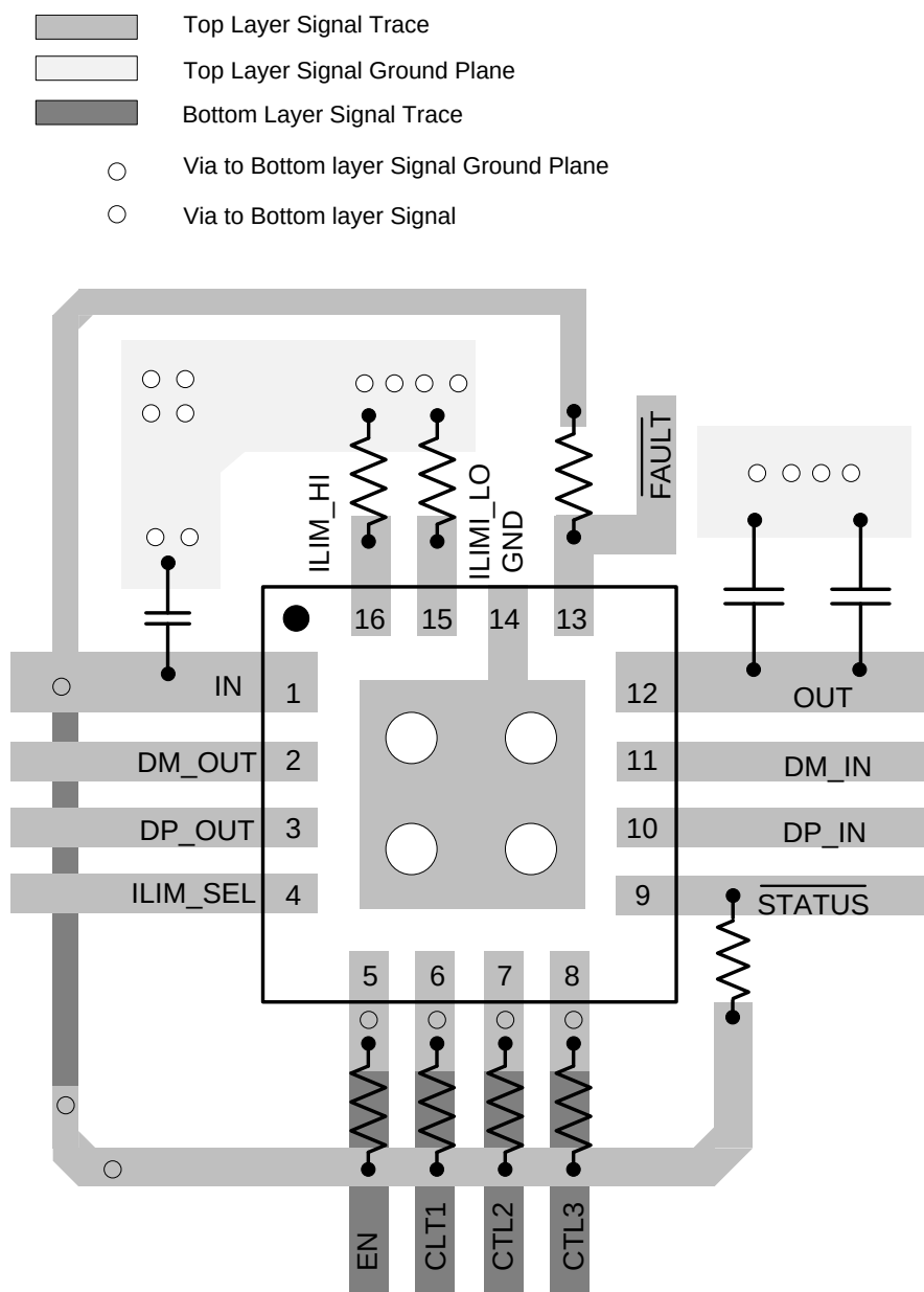
Figure 47. Layout Recommendation
