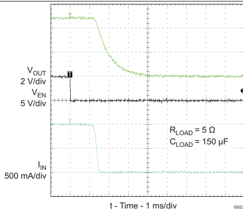
Figure 19. Turnoff Response
