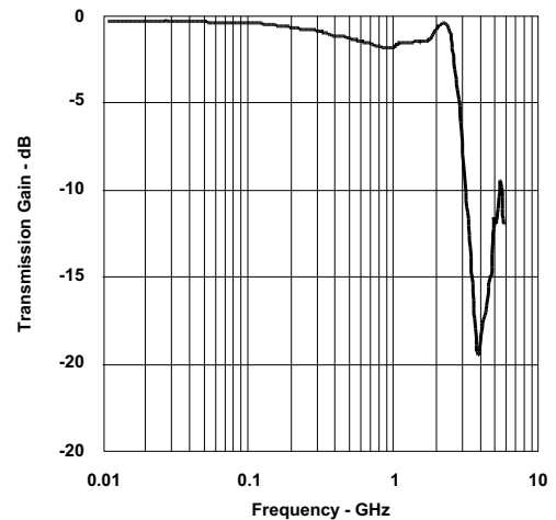
Figure 10. Data Transmission Characteristics vs Frequency
