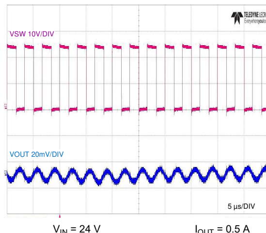
图 7-15. Full-Load Switching
