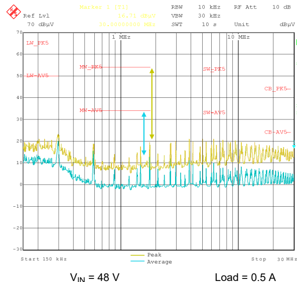
图 7-16. CISPR 25 Class 5 Conducted Emissions Plot, 150 kHz to 30 MHz
