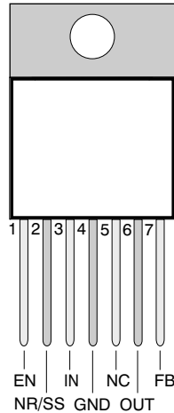
KC Package 7-Pin TO-220 Top View
