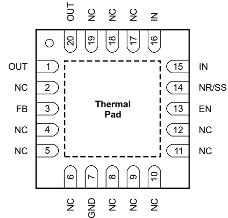
RGW Package 20-Pin VQFN Top View
