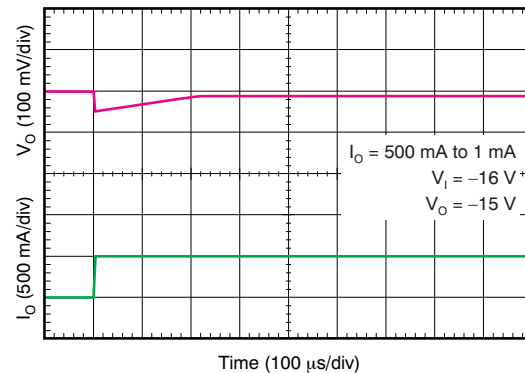
Figure 36. Load Transient
