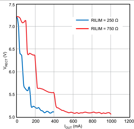
图 7-5. Impact of Maximum Current setting ( R_{ILIM} ) on Rectifier Voltage ( V_{RECT} )
