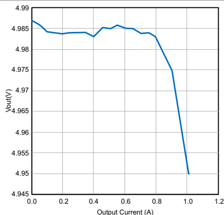
图 7-6. Impact of Load Current on Output Voltage
