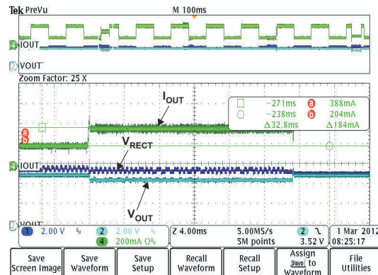
图 7-18. Adaptive Communication Limit Event Where the 400 mA Current Limit is Enabled ( I_{OUT-DC} < 300 \text{ mA} )
