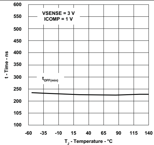
Figure 14. Minimum Off Time vs Temperature
