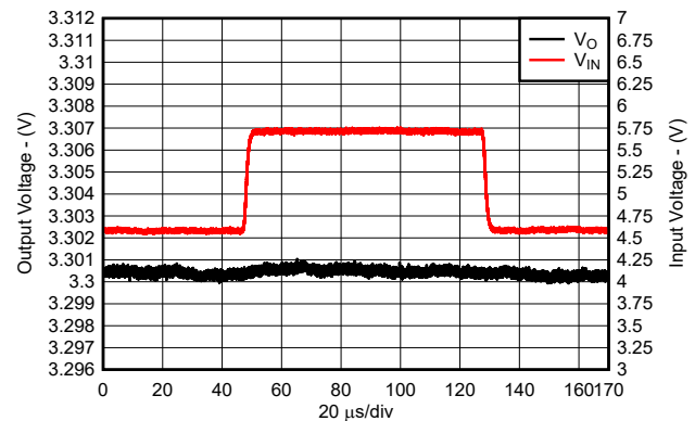
图 7-17. Line Transient Response (New Chip)
