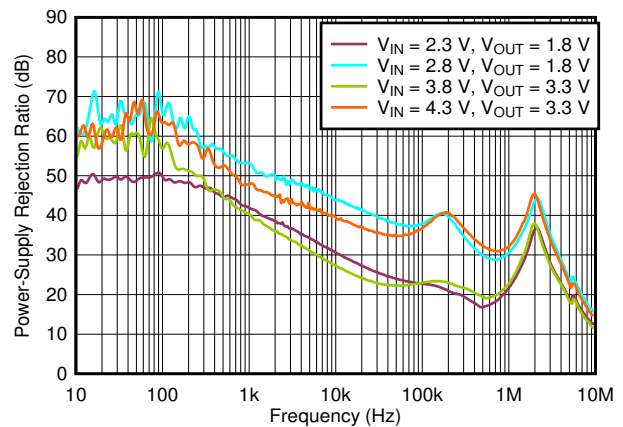
图 5-34. PSRR vs Frequency and V_{IN}
