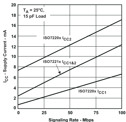
图 5-2. 3.3-V RMS Supply Current vs Signaling Rate (Mbps)
