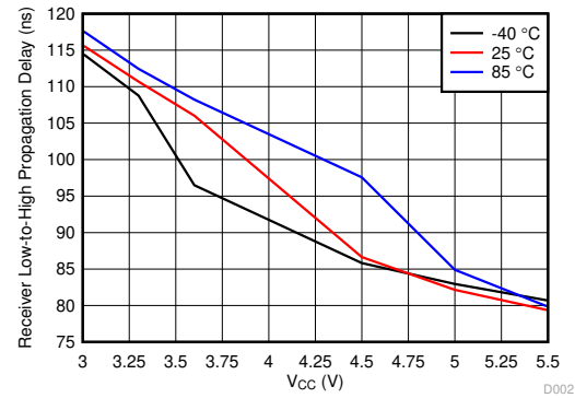
图 5-2. Receiver Path Low-to-High Propagation Delay vs T_A and Supply Voltage (RGT Package)
