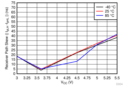
图 5-4. Receiver Pulse Skew ( |t_{pLH} - t_{pHL}| ) vs T_A and Supply Voltage (RGT Package)
