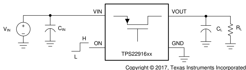
图 9-1. Typical Application
