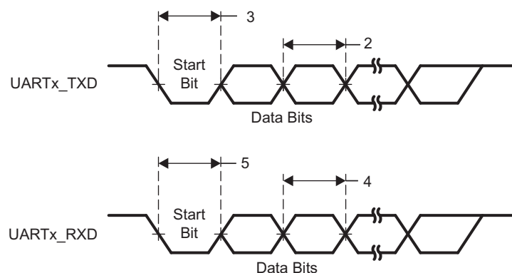
Figure 8-89. UART Timing
