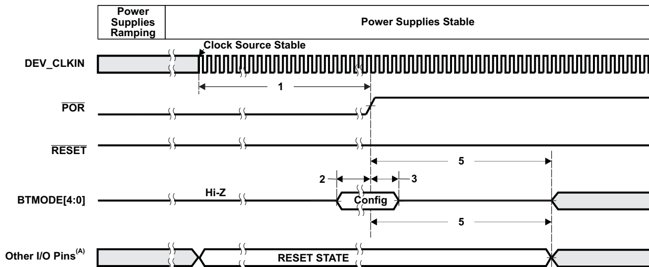
Figure 7-2. Power-Up Timing
