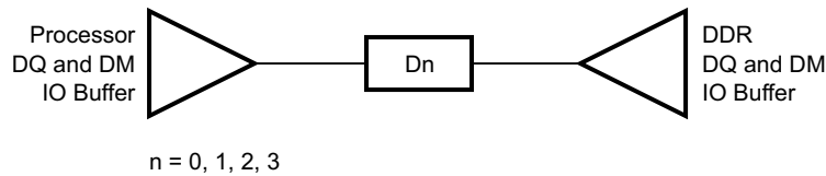
Figure 8-34. DQ/DM Topology
