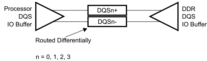
Figure 8-33. DQS Topology
