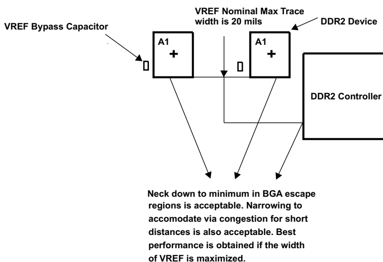
Figure 8-9. VREF Routing and Topology
