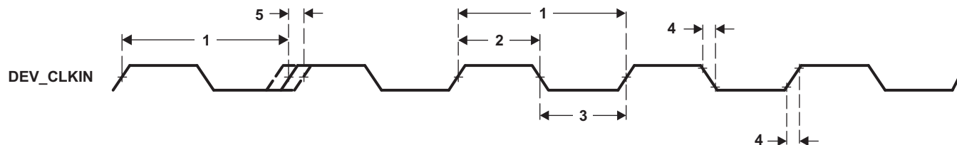
Figure 7-6. DEV_CLKIN Timing
