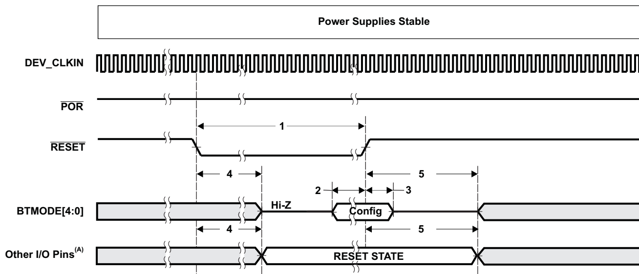
Figure 7-2. Power-Up Timing
