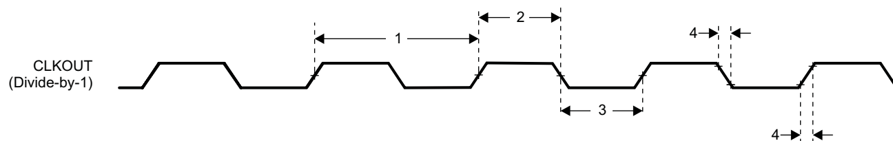
Figure 7-10. CLKOUT Timing
