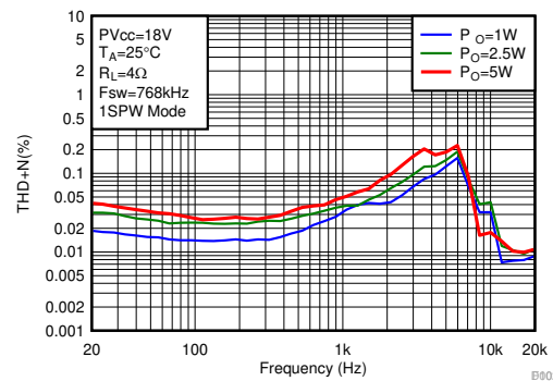
图 6-2. THD+N vs Frequency-BTL
