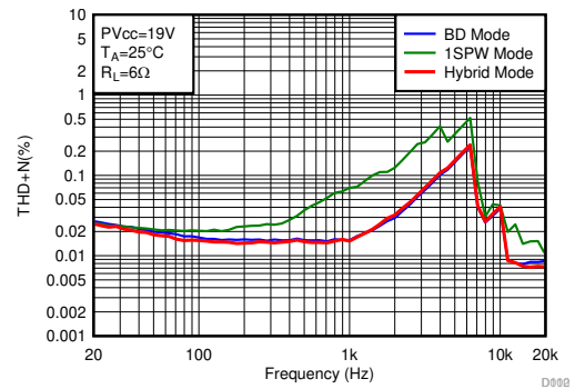
图 6-10. THD+N vs Frequency-BTL
