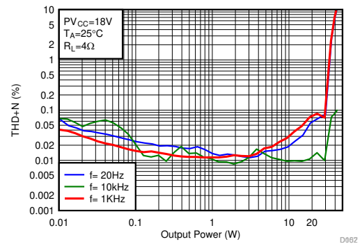
图 8-11. THD+N vs Output Power (Inductor as Output Filter, Hybrid Modulation, PBTL mode)
