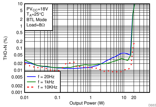
图 6-47. THD+N vs Output Power
