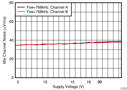
图 6-25. Idle Channel Noise vs PVDD-BTL
