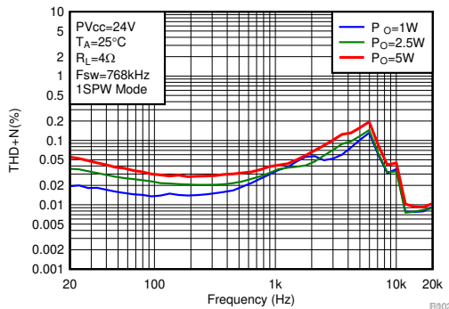
图 6-3. THD+N vs Frequency-BTL
