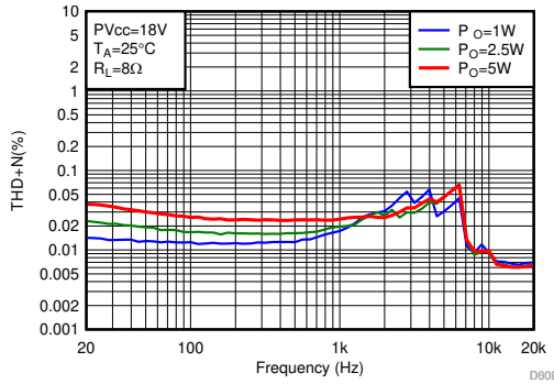
图 6-41. THD+N vs Frequency
