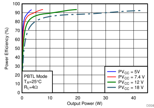
图 6-84. Efficiency vs Output Power
