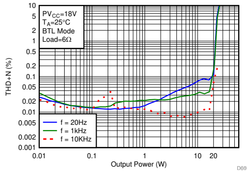
图 6-43. THD+N vs Output Power
