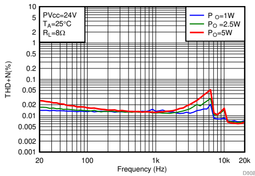
图 6-9. THD+N vs Frequency-BTL
