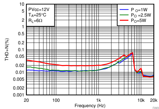
图 6-4. THD+N vs Frequency-BTL
