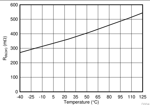
TPS610981 MODE = High / Low
