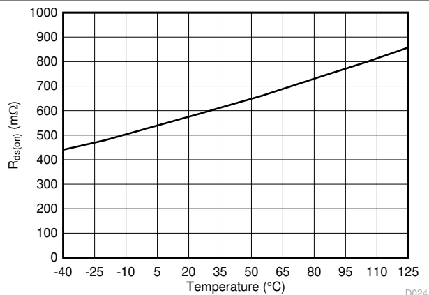
TPS61098, '7 MODE = Low
