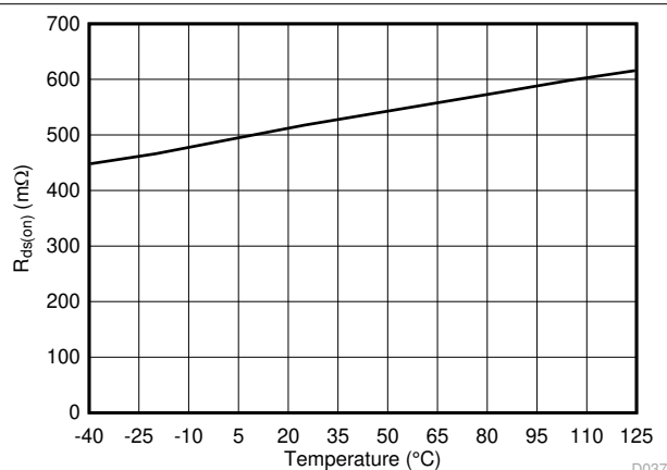
TPS610982 MODE = High / Low
