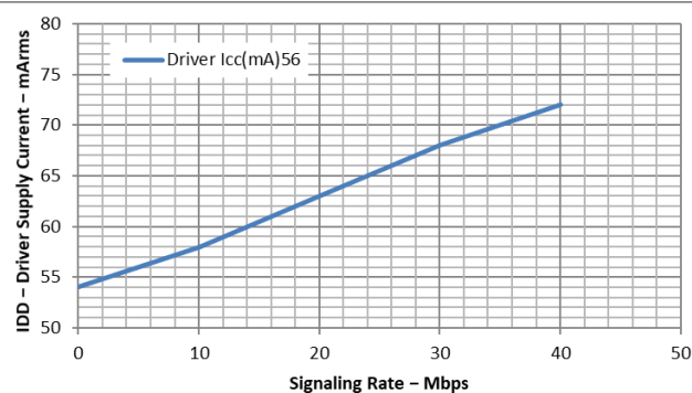
图 6-2. Driver Supply Current vs Signaling Rate
